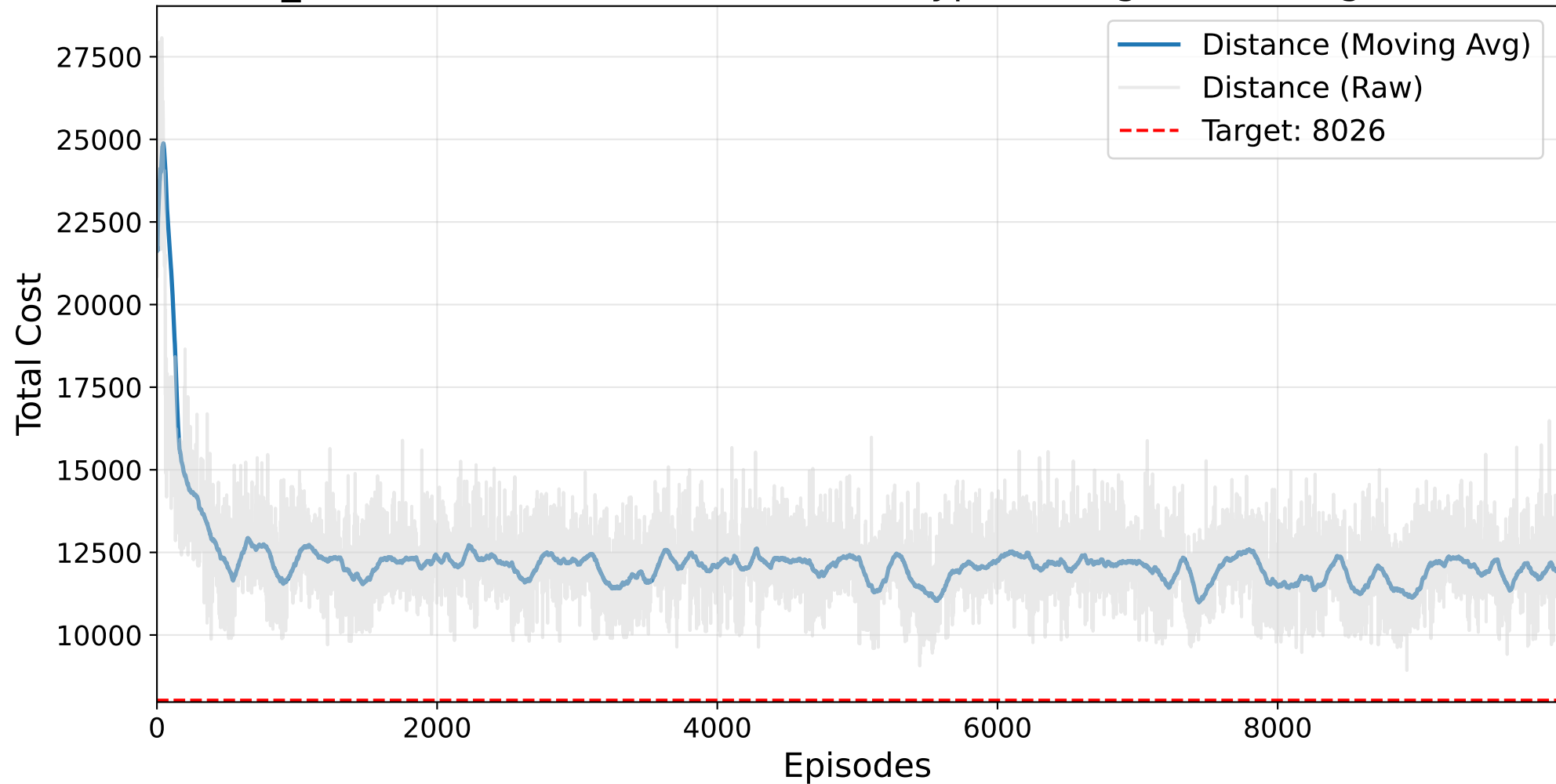
Final NO_BAYESIAN Masked AutoRL-SOP (HyperTuningSK) Training - ft53.2.sop
